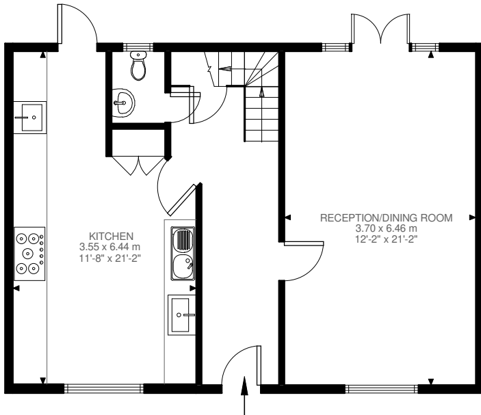
Ground Floor 623 ft²
